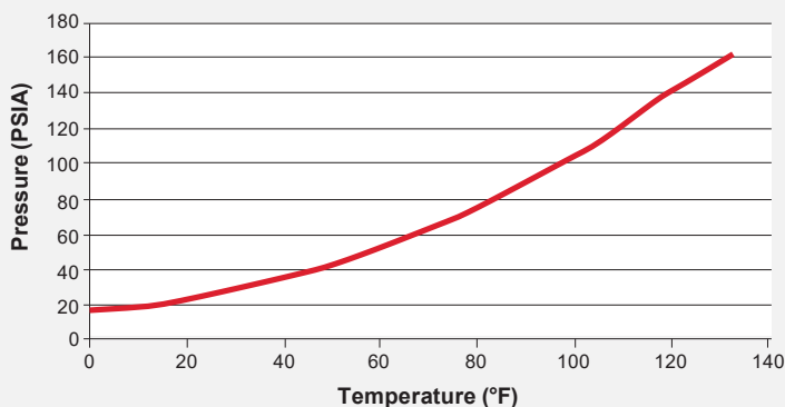
Vapor Pressure vs. Temperature – English Units
